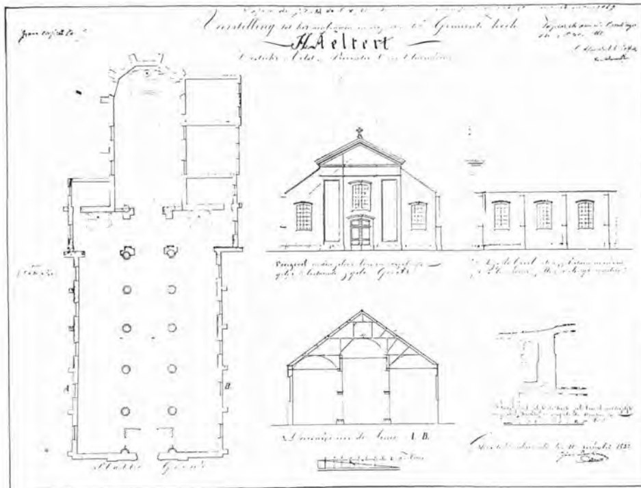
Afb. 1 — Plan 1837 van architect J. Beeckman
